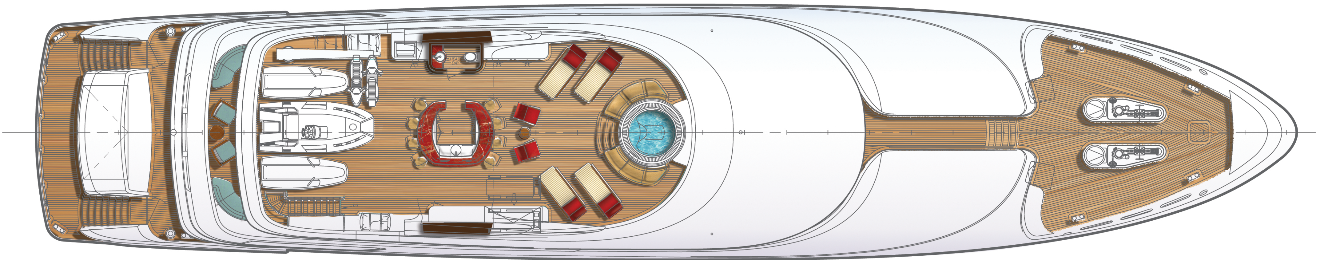
SUN DECK
