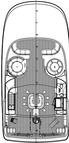
FLYBRIDGE DECK
