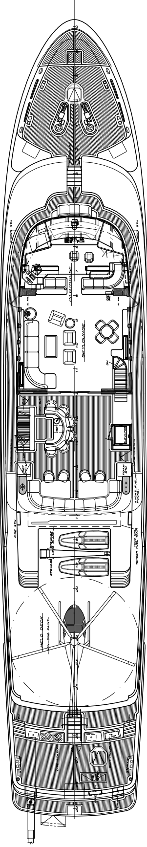
UPPER DECK
