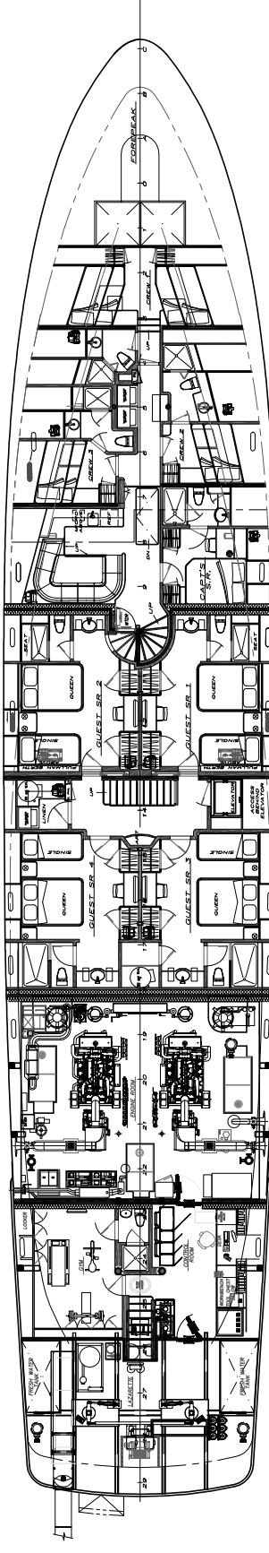
LOWER DECK
