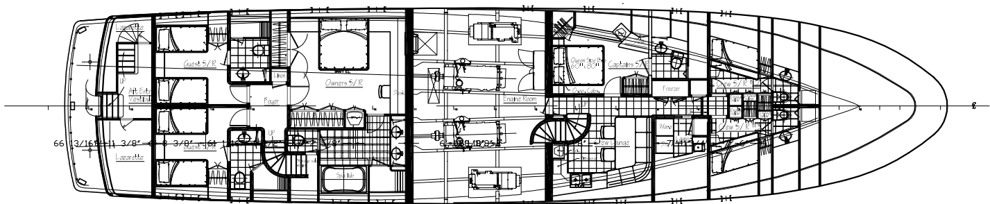
LOWER DECK
