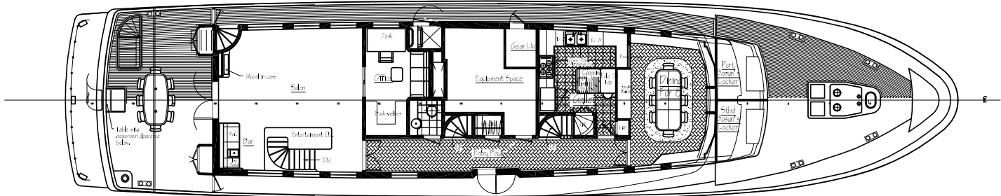
MAIN DECK
