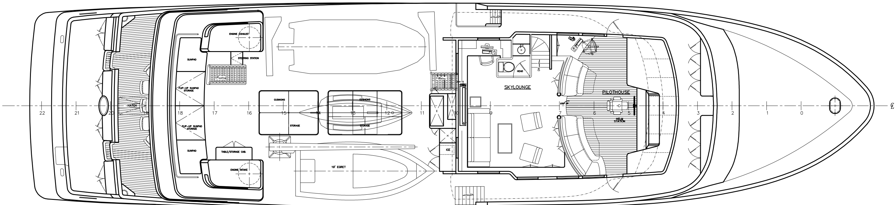
UPPER DECK
