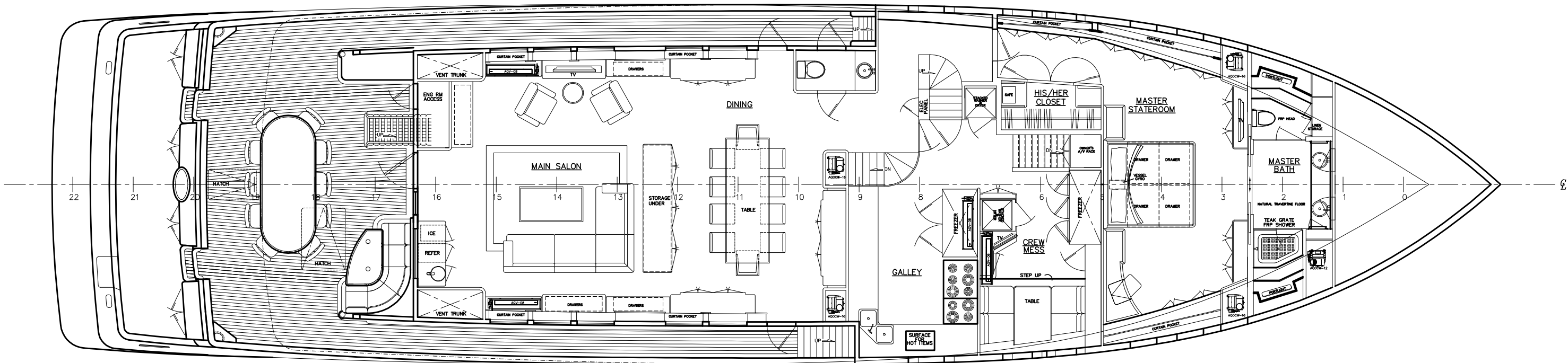
MAIN DECK
