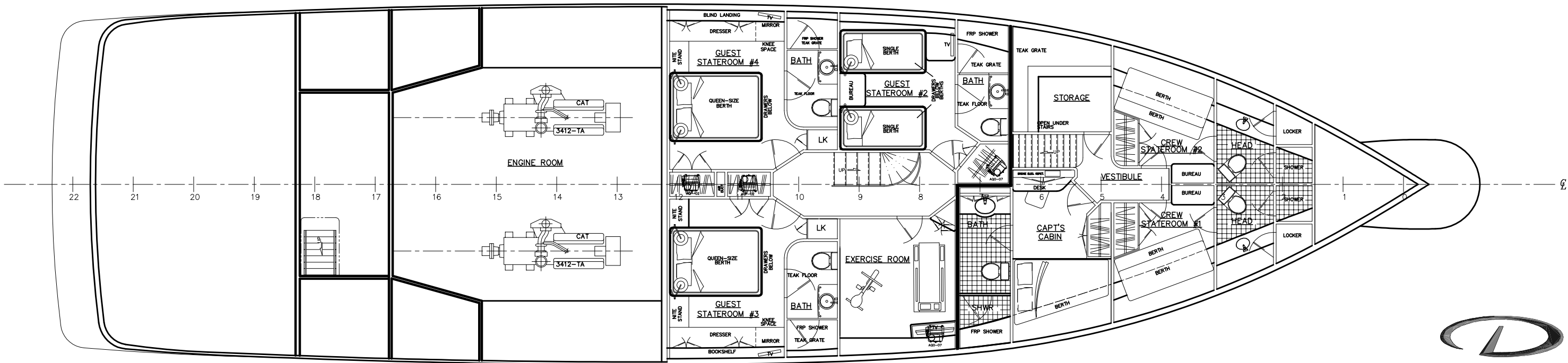
LOWER DECK
